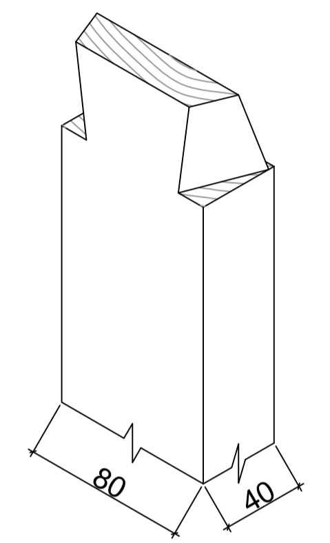
Isometric Detail of vertical support- joint A
