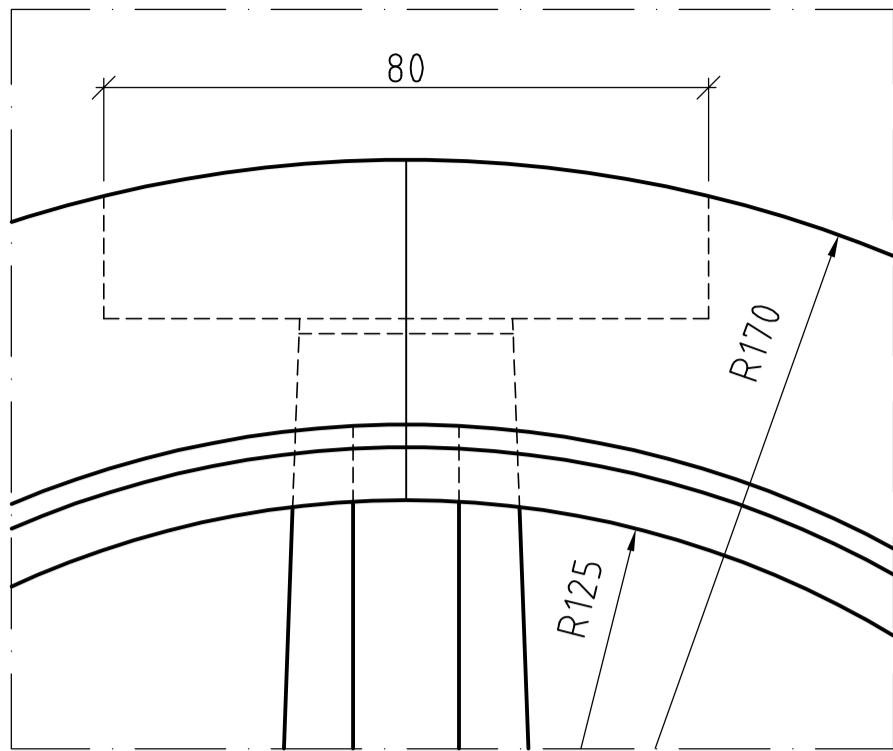
DETAIL 1
