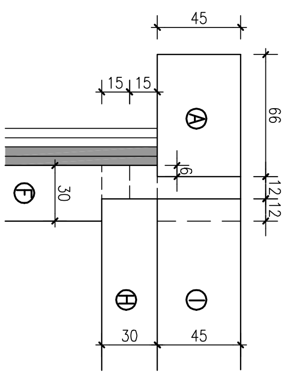
DETAIL G
