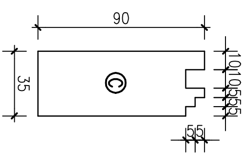
SECTION E-E
