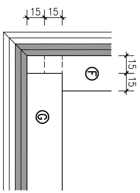
SECTION I-I
