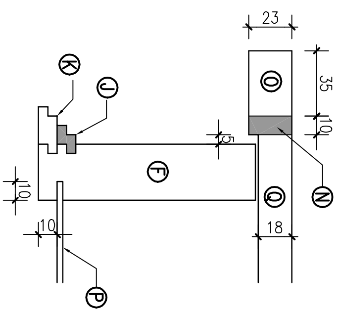
DETAIL F
