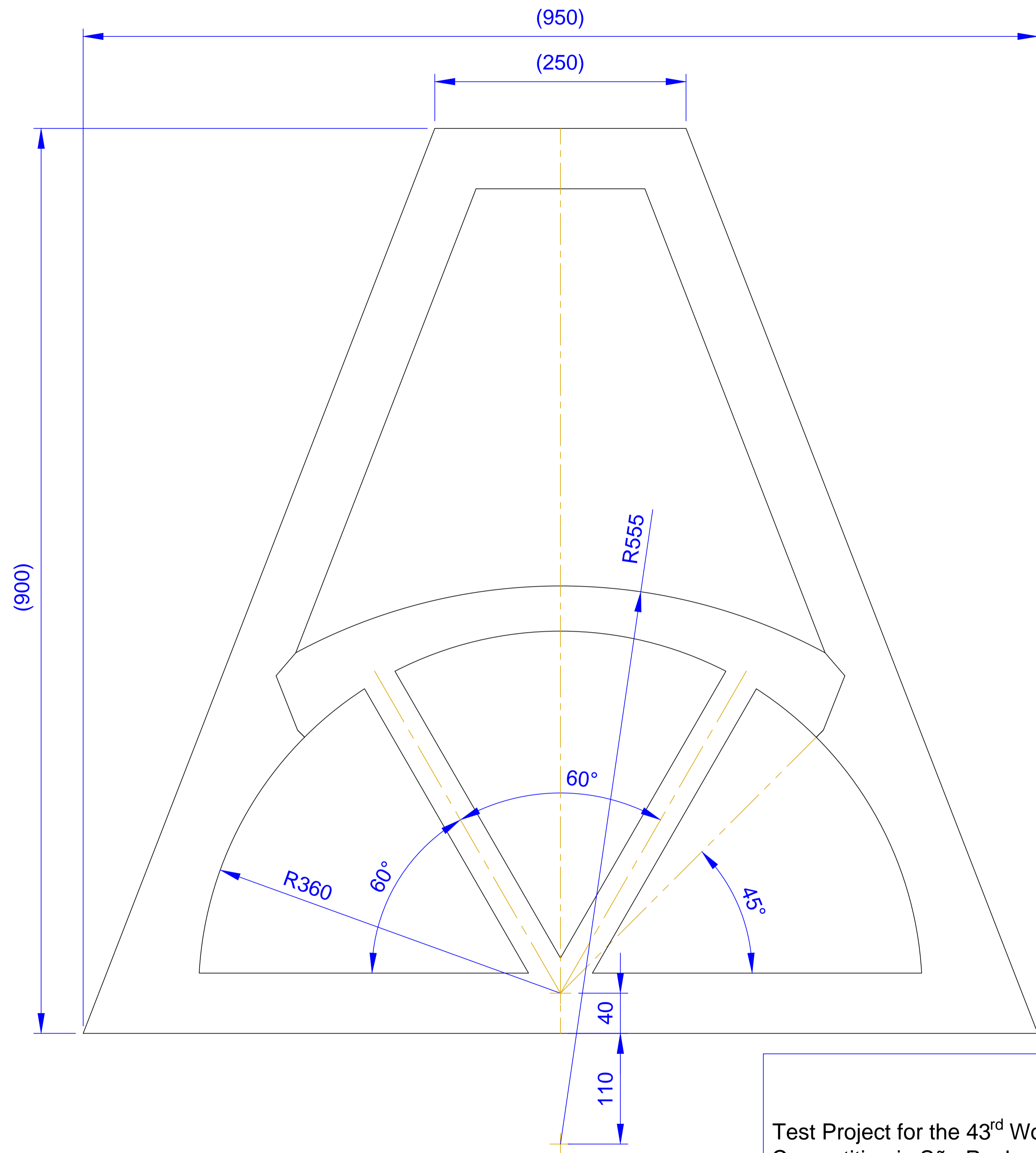
CENTRE POINTS - KEY SETTING OUT
