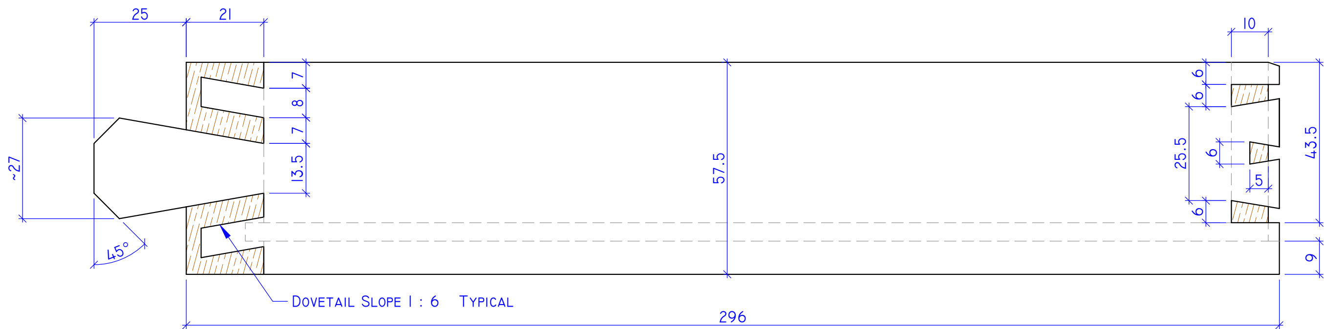
DRAWER DETAIL SCALE 1 : 1
