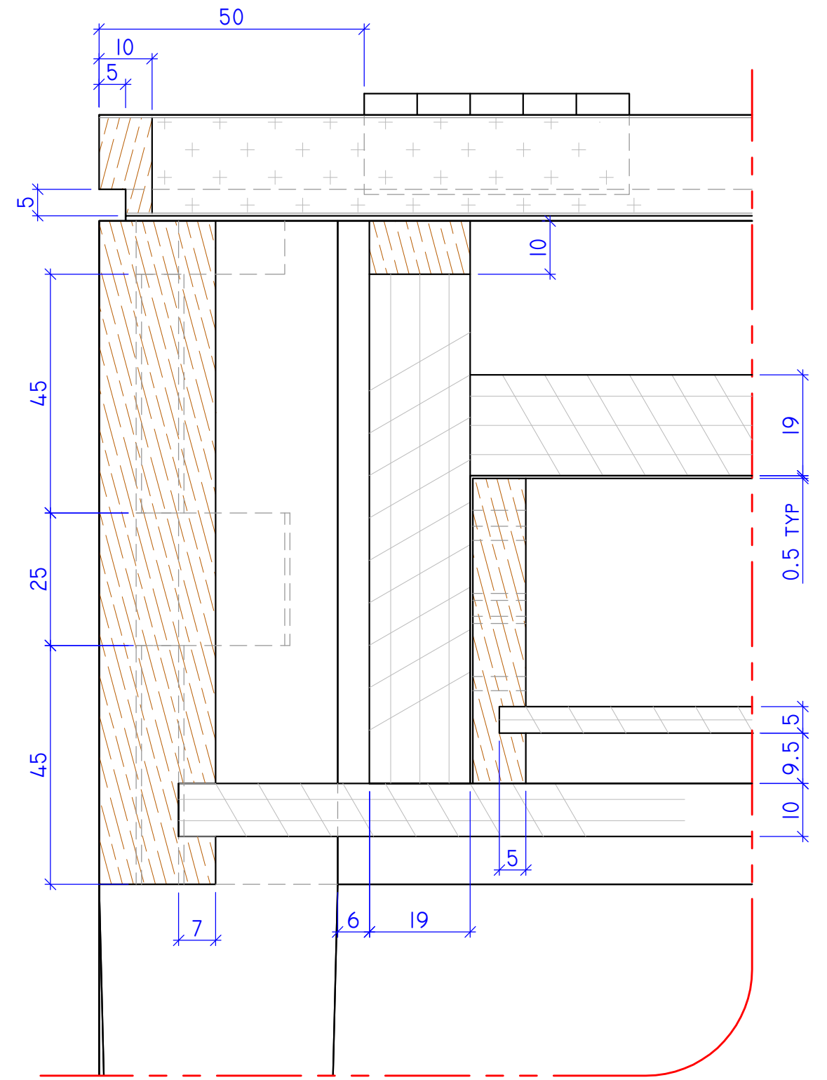
DETAIL 4 SCALE 1 : 1
