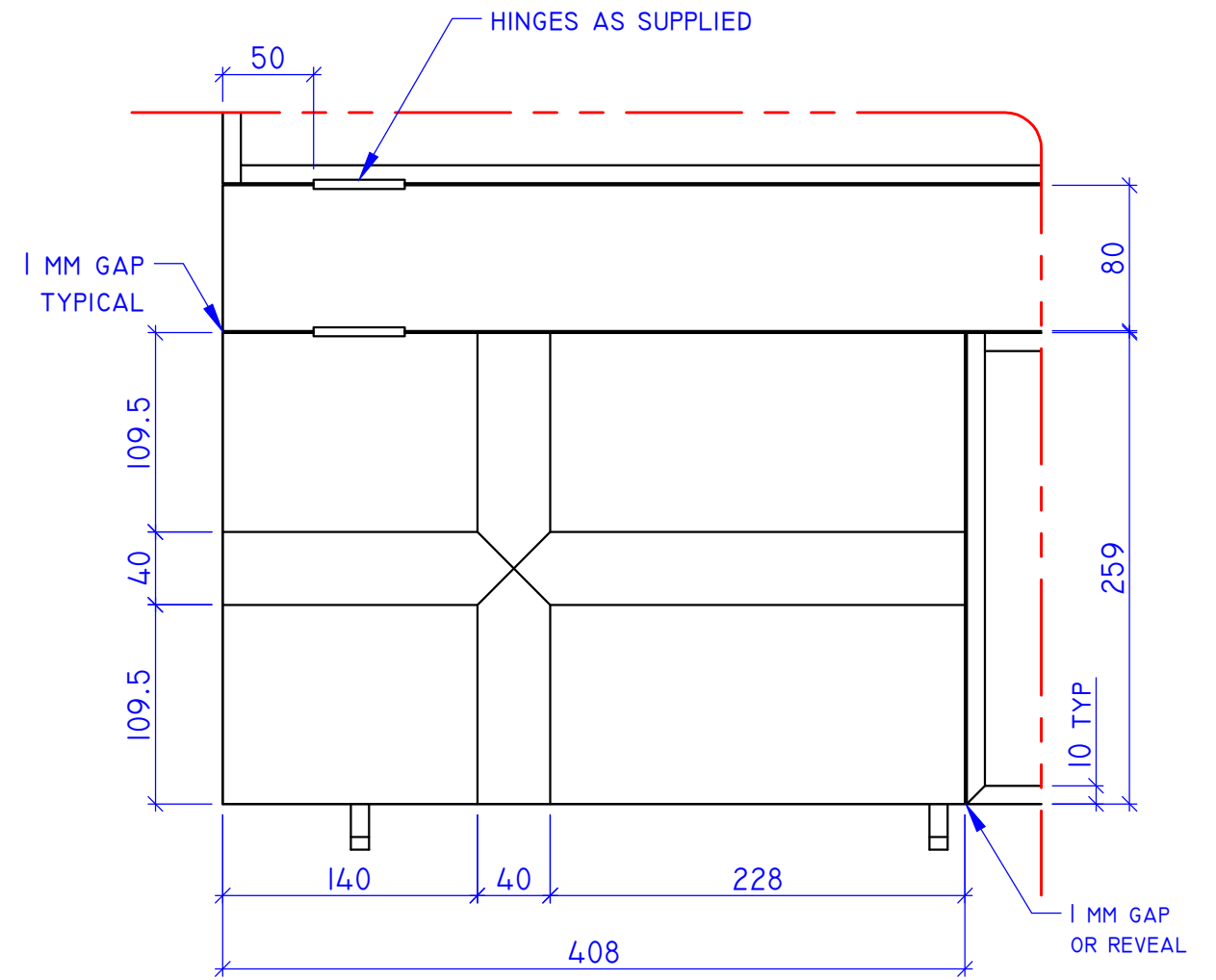
DETAIL I SCALE 1 : 4
