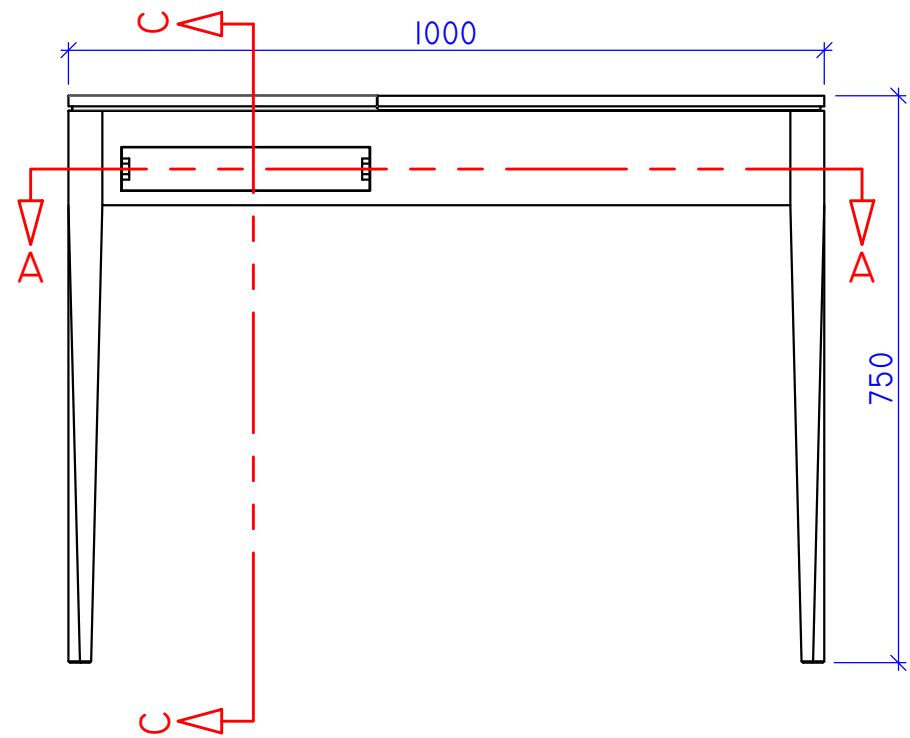
TOP, FRONT AND RIGHT SIDE VIEWS
